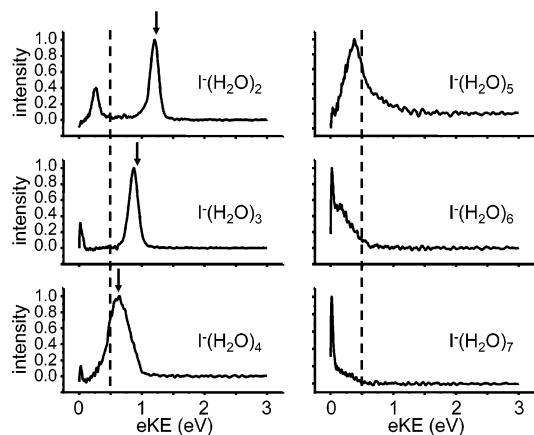
Figure 1. PES of \Gamma^-(\text{H}_2\text{O})_n taken at 5.14 eV. Dotted lines mark e\text{KE} = 0 eV for the pump laser pulse (4.65 eV) used in the time-resolved experiments reported here. Downward arrows mark the maximum of the CTTS absorbance taken from Serxner et al. 4
