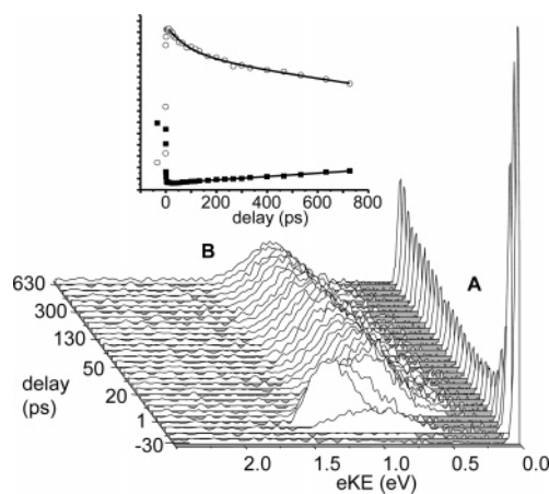
Figure 4. Time-resolved photoelectron spectrum of \Gamma^-(\text{D}_2\text{O})_9 . Signal intensity is plotted as a function of e\text{KE} along the horizontal axis, with pump-probe delay increasing front to back. The inset shows the integrated intensities of features A (filled squares) and B (open circles) as a function of pump-probe delay with fits superimposed as solid lines.
